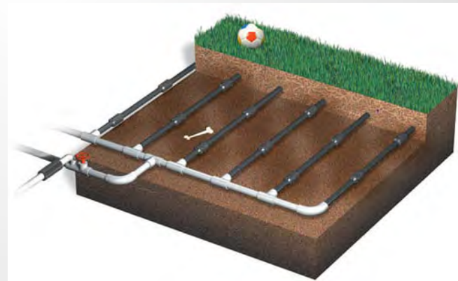
SUBSURFACE DRIP IRRIGATION SYSTEM
